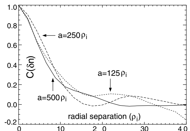
FIG. 1. Radial correlation functions for density perturbations.
