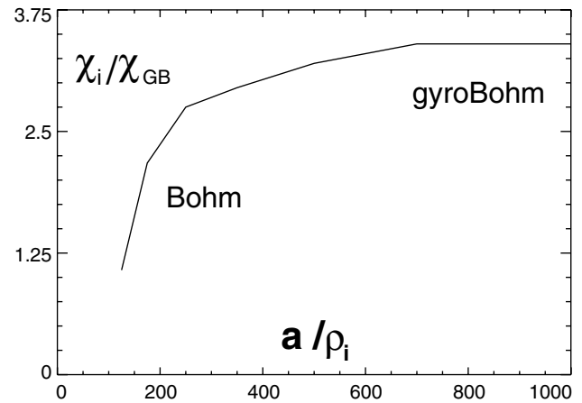
FIG. 3. Ion heat conductivity vs tokamak minor radius.
