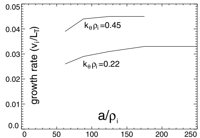
FIG. 4. Linear growth rate vs device size.
